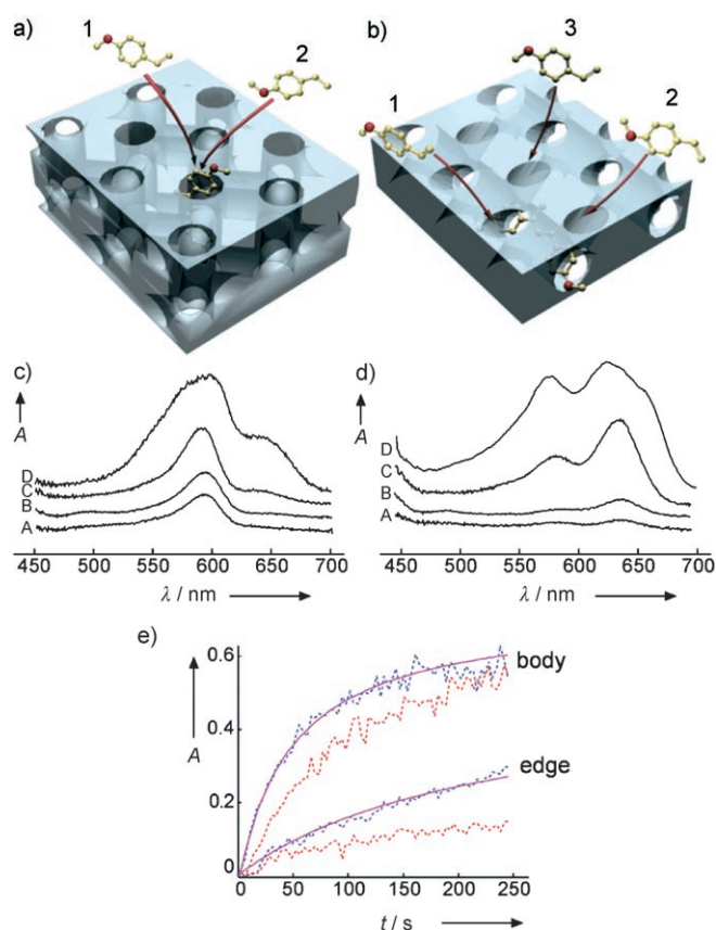
Figure 4. a) Reaction pathways at the edge region: upon formation of the dimerization product (1 + 2), the straight pores are not accessible any more. b) The same as (a), but for the body region: zigzag pore openings adjacent to the reaction site provide access for monomer molecules (3) to diffuse inside and to react with the dimer. c,d) Concentration dependence of the absorption spectra at the edge and the body regions, respectively. The concentration of styrene in hexane solution is A) 36, B) 63, C) 83, and D) 100 wt%. e) Time evolution of the optical absorption at 590 nm (blue) and 635 nm (red). The 590-nm profiles are fitted using second-order kinetic equations (magenta) as described in the text.
