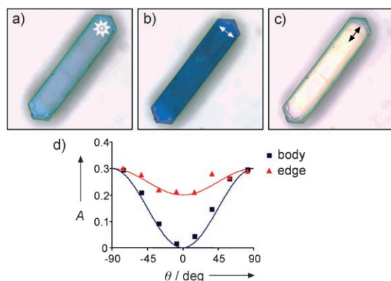
Figure 3. Microphotographs of H-ZSM-5/4-methoxystyrene taken with a) nonpolarized light (star) and b, c) polarized light; polarization is indicated by arrows. d) Angular dependence of the optical absorption at 590 nm, at the body (blue) and edges (red) of the crystal, which follows the \sin^2\theta law, where \theta is the angle between the light polarization vector and the long axis of the crystal.
