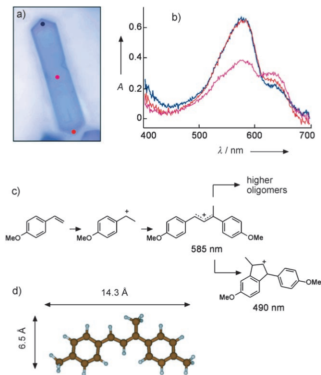
Figure 2. a) Optical microphotograph of a ZSM-5 crystal after addition of 4-methoxystyrene, which demonstrates the different colors observed at the body (blue) and edges (purple). b) Spatially resolved optical absorption spectra measured along the long axis of the crystal after reaction with 4-methoxystyrene at the edges (red and blue) and the center (pink). c) Reaction pathways of 4-methoxystyrene in the acidic zeolite; a neutral styrene molecule is protonated on a Brønsted acid site to form a carbocation, which reacts with another styrene molecule. The dimeric cation may undergo cyclization or react further. d) Calculated molecular geometry of the dimeric carbocation.
