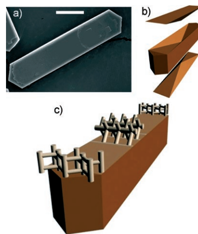
Figure 1. a) Scanning electron microscopy image of a ZSM-5 crystal (size 100 \times 20 \times 20 \mu\text{m}^3 ). Scale bar: 20 \mu\text{m} . b) “Exploded” representation of the crystal showing the individual building subunits. c) Zeolite channel alignment in the different regions of the crystal. The inner zeolite framework, which comprises intersecting straight and zigzag channels, is accessible from the outer surface through openings of the straight pores at the edges and zigzag pores at the body of the crystal.
